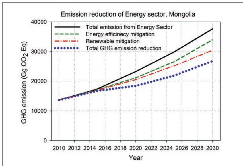
Figure 3-6: Total GHG emission reduction from energy sector
