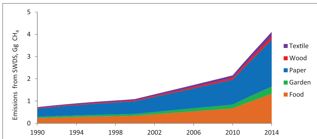
Figure 7-3: Quantities of CH 4 emission from biodegradable solid waste disposed in landfills 1990–2014, Gg
