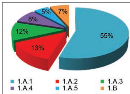
Figure 3-2: The share of aggregated GHG emissions by categories within energy sector in 2014
